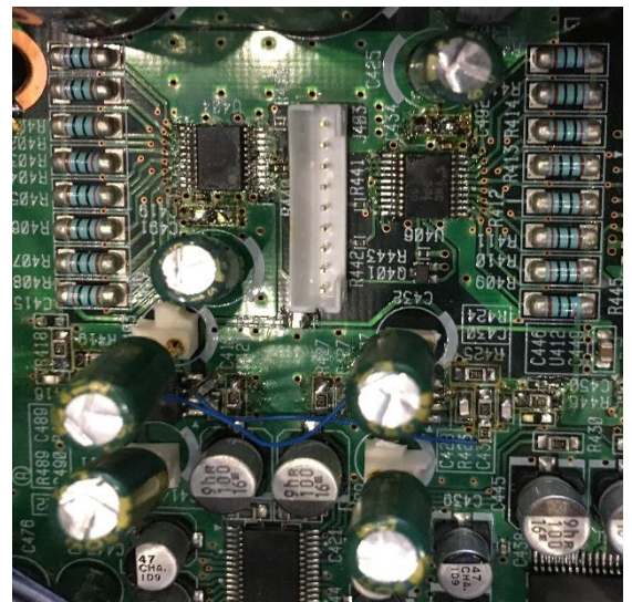
Discrete DAC section (Photo of a prototype)
